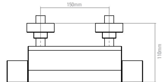
Round Exposed Thermostatic Shower Valve shown
